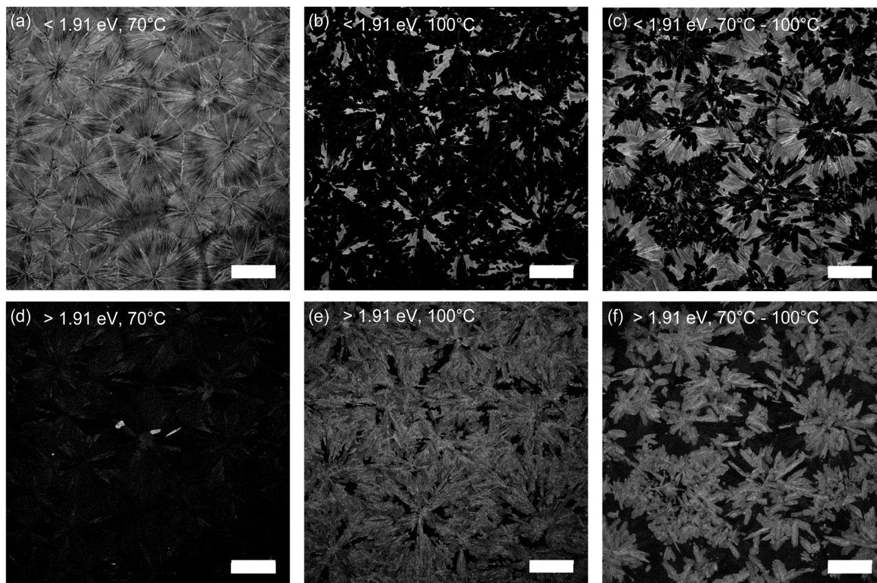
Fig. 4 Confocal photoluminescence micrographs in the range < 1.91 eV (a–c) and > 1.91 eV (d–f) for \text{OBESnI}_4 thin films processed at 70 °C, 100 °C, and 70 – 100 °C. Scale bar is 100 \mu\text{m} .
