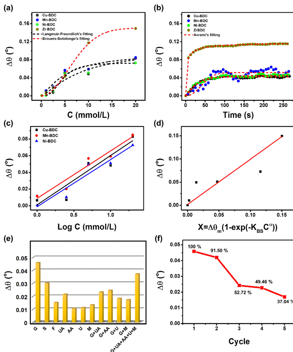
Fig. 4 (a) Non-linear regression curves of Langmuir–Freundlich adsorption isotherm models for glucose-M-BDC ( M = \text{Cu} , \text{Mn} , and \text{Ni} ) and Brouers–Sotolongo for glucose-Zr-BDC. (b) Non-linear regression curves of the Avrami adsorption kinetic models for glucose-M-BDC ( M = \text{Cu} , \text{Mn} , \text{Ni} , and \text{Zr} ). (c) Calibration curves of the dynamic responses of the M-BDC-functionalized SPR sensors towards glucose: Cu-BDC (black), Mn-BDC (red), and Ni-BDC (blue) are obtained by applying linear fitting to the \Delta\theta vs. \log C plots (Langmuir–Freundlich model), and (d) Zr-BDC is obtained by applying linear fitting to the \Delta\theta vs. X = \Delta\theta_m [1 - \exp(-K_{BS} C^\alpha)] plots (Brouers–Sotolongo model). (e) Bar diagrams showing the angular changes of the Zr-BDC-functionalized SPR sensor upon exposure to various molecules [5 mM glucose (G), 5 mM sucrose (S), and 5 mM fructose (F), 0.45 mM uric acid (UA), 0.11 mM ascorbic acid (AA), 5 mM urea (U), and 0.1 mM maltose (M)]. (f) The corresponding percentage of the dynamic response of Zr-BDC-functionalized SPR sensor to 5 mmol L -1 glucose after the n th measurement compared to the first measurement.
