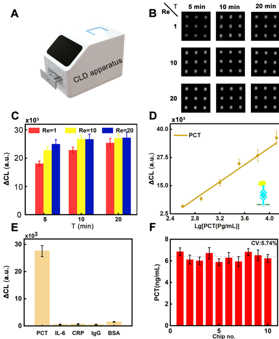
Fig. 6 (A) Chemiluminescence detection apparatus, PCT concentration of 3.2 ng mL -1 at different Re and incubation times for dot signal (B) and corresponding \Delta\text{CL} intensity (C). (D) Standard curve between the PCT concentration and \Delta\text{CL} intensity ( N = 3 ). (E) The selectivity assay of the developed for detection of PCT. (F) The stability research of the chips (No. 10) for PCT (6.4 ng mL -1 ) analysis.
