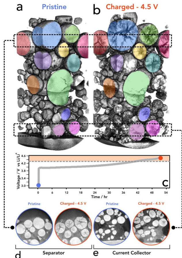
Fig. 1 (a and b) Volume rendering of the same region of an NMC811 electrode at (a) blue – pristine and (b) red – charged state (4.5 V vs Li/Li + ). (c) Charging profile for NMC811 electrode to 4.5 V at C/50, noting potentials at which the two nano-CT datasets were collected. (d and e) Representative ortho slices of the same particles at pristine and charged state at (d) separator and (e) current collector.
