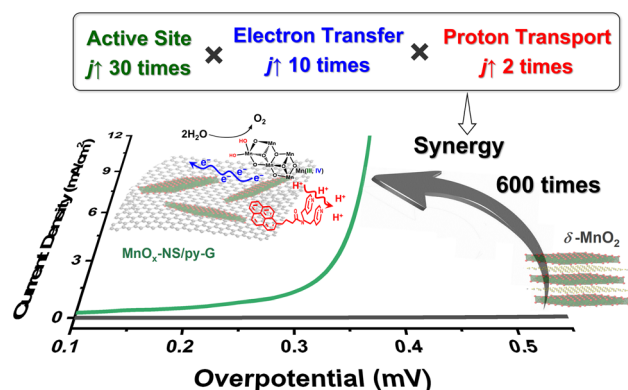
Scheme 3 Schematic illustration of the origin of the dramatic activity enhancement owing to the synergy of catalytically active site exposure, fast electron transport, and efficient proton transport.
