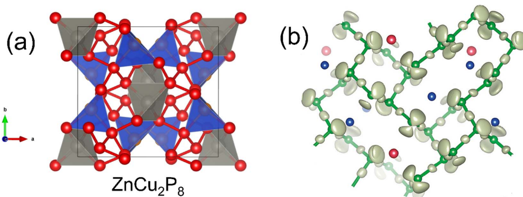
Fig. 3 Crystal structure of \text{ZnCu}_2\text{P}_8 . Panel (a) shows the tetrahedral coordination of Zn (grey), Cu (blue) and the P–P network (red). Panel (b) shows the lone pair behavior of P (green), where P atoms with one lone pair coordinate to Cu (blue), and P atoms with 2 lone pairs bond to Zn (red). Panel (b) reproduced with permission from Nuss et al., Zeitschrift für Anorganische und Allgemeine Chemie , 2020. 63
