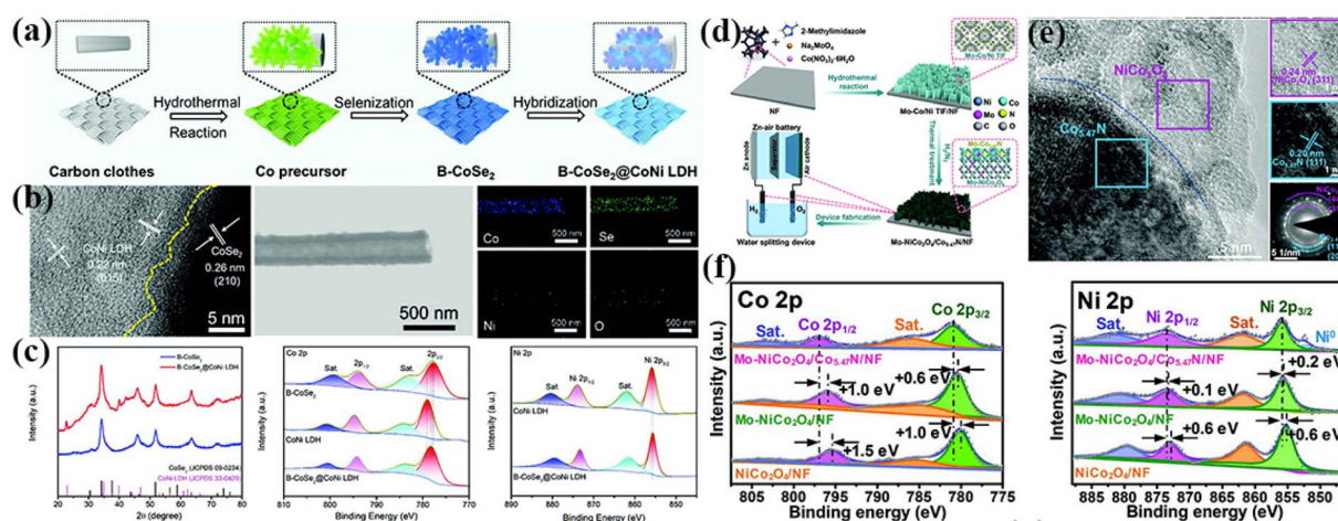
Fig. 7 (a) Schematic illustration of the synthetic process of \text{B-CoSe}_2@/\text{CoNi} LDH HNA. (b) HRTEM image of \text{B-CoSe}_2@/\text{CoNi} LDH HNA highlighting the interface between \text{CoSe}_2 and \text{CoNi} LDH and elemental mapping images of \text{B-CoSe}_2@/\text{CoNi} LDH HNA. (c) XRD spectra and XPS patterns for \text{B-CoSe}_2 , \text{CoNi} LDH, and \text{B-CoSe}_2@/\text{CoNi} LDH HNA. Reproduced with permission from ref. 152, Copyright (2022) Wiley. (d) Schematic illustration of the synthetic process of \text{Mo-NiCo}_2\text{O}_4/\text{Co}_{5.47}\text{N}/\text{NF} . (e) HRTEM images and SAED pattern of \text{Mo-NiCo}_2\text{O}_4/\text{Co}_{5.47}\text{N}/\text{NF} . (f) XPS spectra of \text{Mo-NiCo}_2\text{O}_4/\text{Co}_{5.47}\text{N}/\text{NF} , \text{Mo-NiCo}_2\text{O}_4/\text{NF} , and \text{NiCo}_2\text{O}_4/\text{NF} . Reproduced with permission from ref. 154, Copyright (2020) Wiley.
