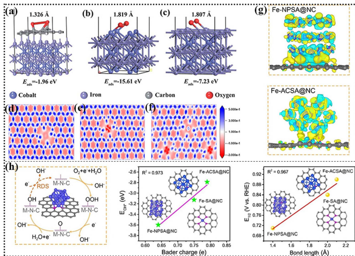
Fig. 11 Adsorption energies ( E_{\text{ads}} ) on the (200) surfaces of CoFe and the optimized geometries of (a) CoFe@NC, (b) CoFe@Co and (c) CoFe@Fe systems. Reproduced with permission from ref. 130, Copyright (2020) RSC. Calculated charge density differences for (d) Zn-N 4 , (e) Cu-N 4 and (f) Cu-N 4 /Zn-N 4 (blue and red areas represent charge density increase and decrease, respectively, where larger values represent increased electron density). Reproduced with permission from ref. 187, Copyright (2021) Wiley. Differential charge density of (g) Fe-NPSA@NC and Fe-ACSA@NC (colors yellow and blue represent the increase and decrease in charge density, respectively). (h) ORR elemental steps in alkaline media and OH* adsorption energy as a function of average Fe. Reproduced with permission from ref. 189, Copyright (2022) Wiley.
