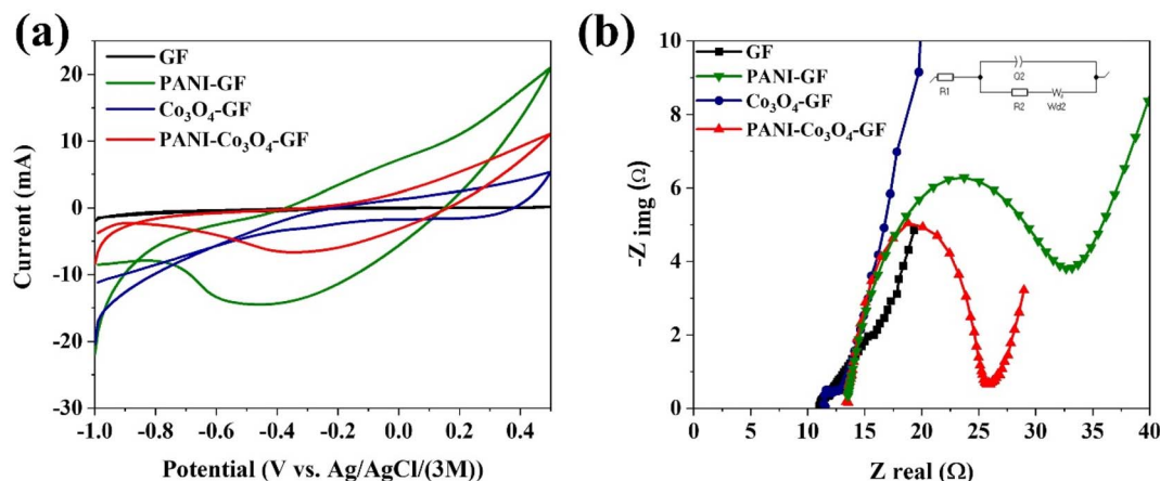
Fig. 4 Electrochemical characterisation of the anode electrodes before use. (a) CV scans at 0.01 \text{ V s}^{-1} and (b) EIS spectra. Tests were performed in a 3-electrode system in 50 \text{ mM PBS (pH 7)} , with the anode as the working electrode and Pt wire (diameter: 0.127 \text{ mm} ) as the counter electrode.
