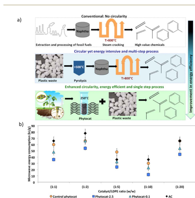
Fig. 8 (a) Schematic illustration of the processes to generate high value chemicals, (b) microwave energy consumption for accelerated de-polymerization of LDPE (to reach the set point of 250 °C) using varying catalyst to polymer ratio.
