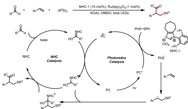
Scheme 7 Synthesis of α-arylated-β-thiolated ketones.
