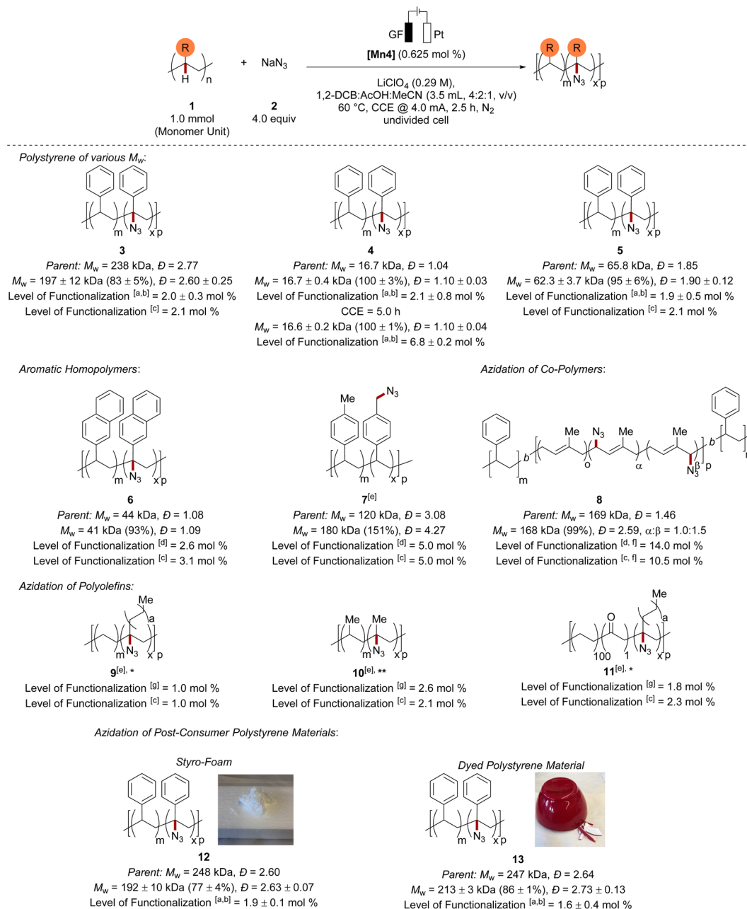
Scheme 1 Scope of the mangana-electrocatalyzed azidation. Standard reaction conditions: 1 (1.0 mmol, 1.0 equiv.), 2 (4.0 mmol, 4.0 equiv.), [Mn4] (6.25 \mu mol), \text{LiClO}_4 (0.29 M), 1,2-DCB (2.0 mL), AcOH (1.0 mL), MeCN (0.5 mL), CCE @ 4.0 mA at 60 °C under \text{N}_2 for 2.5 h. The mass average molar mass and dispersity ( \bar{D} ) were determined by GPC against narrow-disperse polystyrene standards using THF as eluent at 30 °C and were reported as the molar weight retention of the parent polymer. *Reaction performed at 80 °C. **Reaction performed at 120 °C. a The level of functionalization was estimated using an IR- 1 H NMR correlation curve ( m = 2.7051 \text{ mol}\% , R^2 = 0.9942 ) and the relative IR intensity of the \text{N}_3^- band ( 2106 \text{ cm}^{-1} ) to the benzylic C-H band ( 3026 \text{ cm}^{-1} ) of the polystyrene sample. b Results are reported as average over three runs. c The level of functionalization was determined by elemental analysis. d The level of functionalization was determined by 1 H NMR analysis of the 1,3-cycloaddition product with methyl propiolate. e For details on selectivity, see the ESI. f The level of functionalization refers to \alpha and \beta (1.0 : 1.5) in total. g The level of functionalization was estimated by 1 H NMR analysis of the 1,3-cycloaddition product with dimethyl acetylenedicarboxylate.
