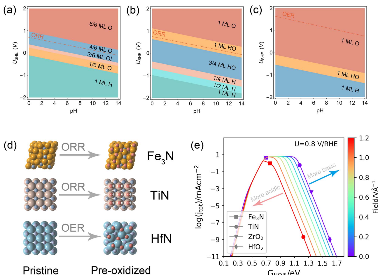
Fig. 6 Calculated 2D surface Pourbaix diagrams as a function of potential (vs. SHE) and pH ( T = 298.15 K) for (a) \text{Fe}_3\text{N}(111) , (b) TiN(100), and (c) HfN(100). (d) Corresponding atomic structures before and after surface state changes. Yellow, brown, cyan, blue, red, and white spheres denote Fe, Ti, Hf, N, O, and H atoms, respectively. (e) Derived pH-dependent volcano activity model for the ORR as a function of \text{HO}^* adsorption (at 0.8 V vs. RHE) plotted with the \text{Fe}_3\text{N}(111) , TiN(100), \text{ZrO}_2(111) , and \text{HfO}_2(111) under their identified surface states under ORR conditions. Note: the pristine surfaces were previously identified to be favorable under ORR conditions for \text{ZrO}_2 and \text{HfO}_2(111) . 19
