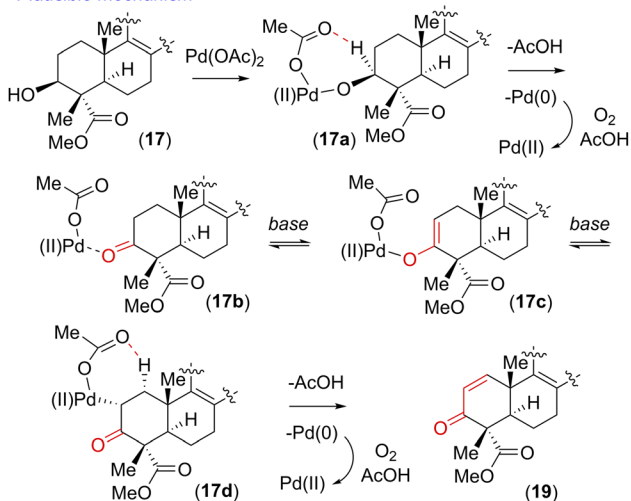
Scheme 5 Plausible mechanism involving overoxidation.
