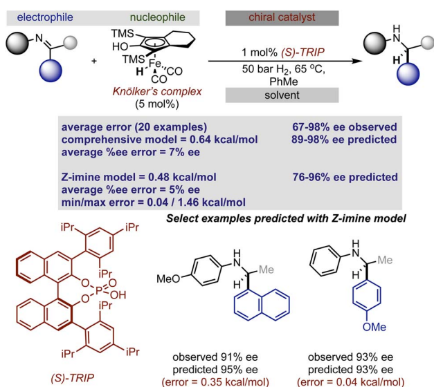
Fig. 3 Extrapolation of a previously reported chiral Brønsted acid imine reaction model to iron catalysed hydrogenation.
