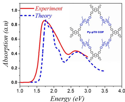
Fig. 4 Comparison of the simulated spectrum using the MHH with the measured absorption spectrum of py-ptII COF replotted from ref. 293.
