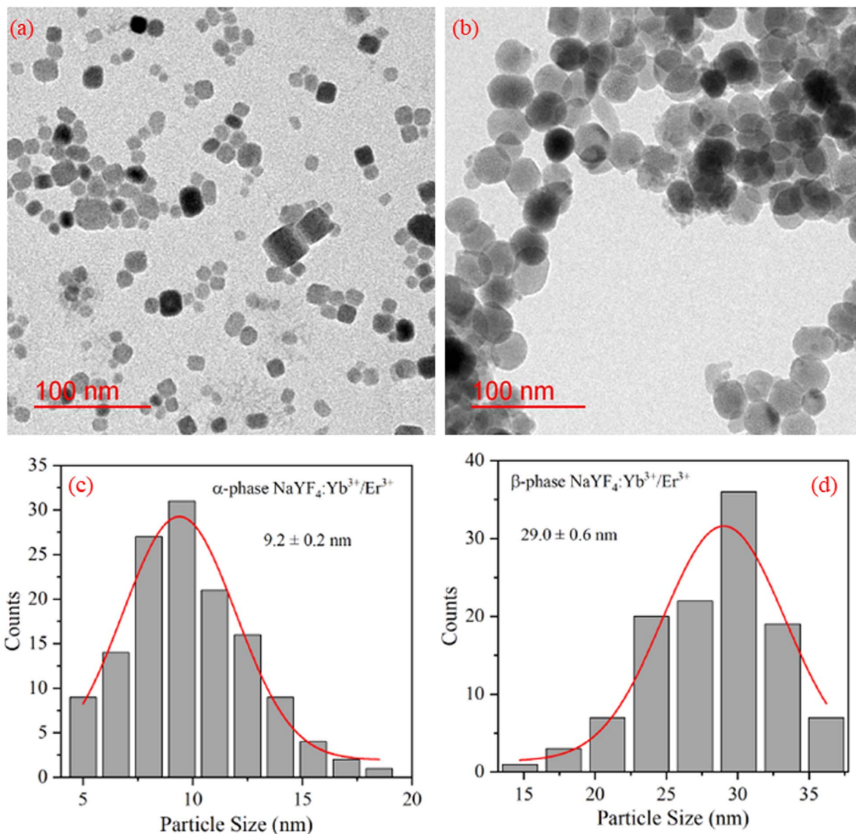
Fig. 2 TEM image of (a) \alpha - \text{NaYF}_4\text{:Yb}^{3+}/\text{Er}^{3+} , (b) \beta - \text{NaYF}_4\text{:Yb}^{3+}/\text{Er}^{3+} nanophosphor. (c) and (d) shows the particle size distribution of \alpha - \text{NaYF}_4\text{:Yb}^{3+}/\text{Er}^{3+} , and \beta - \text{NaYF}_4\text{:Yb}^{3+}/\text{Er}^{3+} nanophosphor, respectively.
