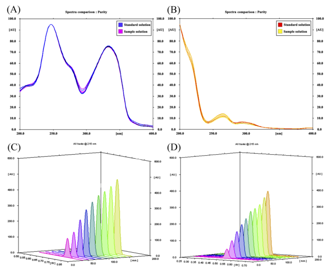
Fig. 3 Superimposed spectrodensitograms for the standard and sample tablet solutions of (A) ALF and (B) SOL for wavelength selection and peak purity assessment. (C and D) Scanning 3D profiles in range of 0.2–8.0 \mu g per band for ALF and 0.1–6.0 \mu g per band for SOL, respectively.
