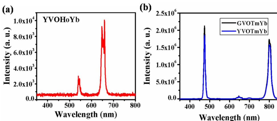
Fig. 4 (a) UC emission spectrum of \text{YVO}_4:\text{Ho}^{3+}, \text{Yb}^{3+} phosphor in the range 350–800 nm. (b) UC emission spectra of \text{Tm}^{3+}/\text{Yb}^{3+} co-doped \text{GdVO}_4 and \text{YVO}_4 phosphors in the range from 350–850 nm. ((b) is reproduced with permission from ref. 32 with copyright 2020, Elsevier).
