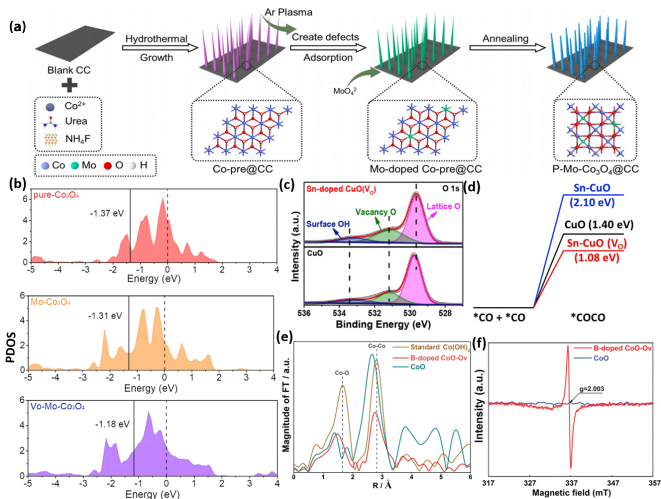
Fig. 13 (a) The figure provides a schematic depiction of the synthesis process for P-Mo-Co 3 O 4 @CC. (b) PDOS of pure-Co 3 O 4 , Mo-Co 3 O 4 , and V 0 -Mo-Co 3 O 4 . Reproduced from ref. 53. (c) XPS O 1s spectra of CuO and CuO that have been doped with Sn (V 0 ). (d) Diagram illustrating the amount of energy required for CO dimerization ( ^*\text{CO} + ^*\text{CO} \rightarrow ^*\text{OCCO} ) on CuO (black), Sn-CuO (blue), and Sn-CuO(V 0 ) (red). Reproduced with permission. 161 (e) The spectra were obtained using the Fourier transform at the Co K-edge for B-doped CoO-OV, CoO, and conventional Co(OH) 2 . (f) Spectra of EPR for B-doped CoO-OV and CoO. Reproduced from ref. 162 with permission from Elsevier, copyright 2021.
