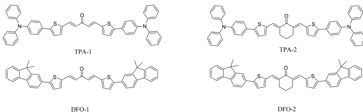
Scheme 1 Chemical structures of the chalcones examined in this study.
