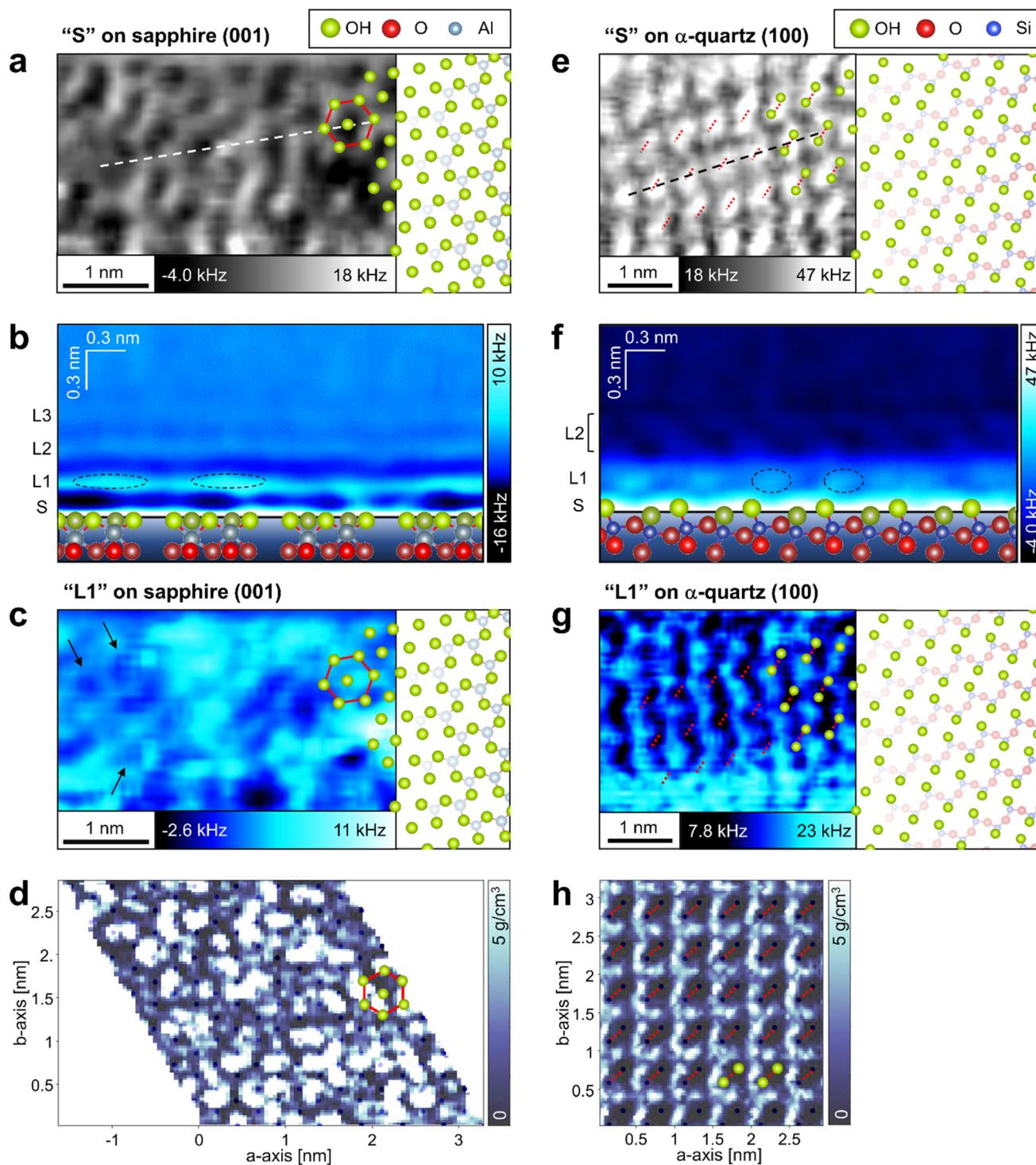
Fig. 4 Local water density distributions on the sapphire (001) and the \alpha -quartz (100) surfaces. (a, c, e, g and h) XY and (b and f) Z cross-sections extracted from (a, b, c, e, f and g) 3D- \Delta f images obtained using 3D-AFM and (d and h) 3D- \rho images calculated using MD simulations for (a–d) sapphire (001) and (e–h) \alpha -quartz (100) surfaces, respectively. The XY cross-sections are extracted at positions (a and e) S and (c, d, g and h) L1 as indicated in Fig. 3b, c, e and f. The Z cross-sections in b and f are extracted along the dotted line in a and e. The hexagonal structure in sapphire (001) and the strongly hydrogen-bonded OH groups in \alpha -quartz (100) are indicated by red lines or dotted lines in a, c, d, e, g and h.
