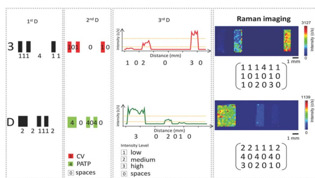
Fig. 7 Intensity encoding for the Raman security label. The information "3D" is stored in the Raman QR code. Reproduced with permission from ref. 44. Copyright 2016 John Wiley & Sons, Inc.
