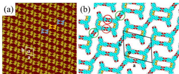
Fig. 1 (a) High-resolution STM image of H 4 BDETP's linear structure at the 1-heptanoic acid/HOPG interface, and the tunneling conditions were: I_{\text{set}} = 216.7 pA, V_{\text{bias}} = 707.4 mV (32.0 nm \times 32.0 nm). (b) The calculated molecular model for the linear structure.
