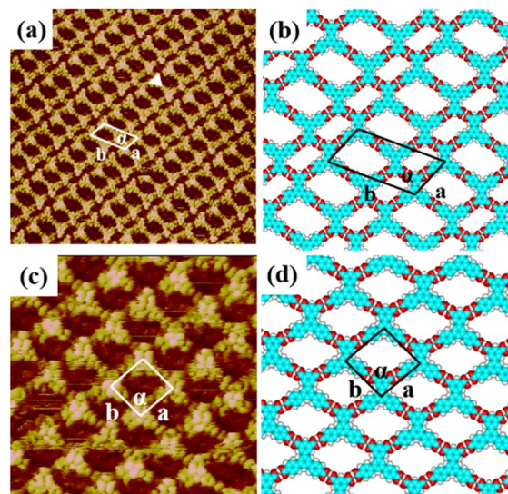
Fig. 2 High-resolution STM image of H 4 BTB's (a) lamellar structure (25 nm \times 25 nm) and (c) tetragonal structure (25 nm \times 25 nm) at the 1-heptanoic acid/HOPG interface both with the tunneling conditions of I_{\text{set}} = 362.2 pA and V_{\text{bias}} = 668.0 mV. (b) and (d) The corresponding optimized molecular packing models for H 4 BTB's lamellar nanostructure in (a) and tetragonal nanostructure in (c) respectively.
