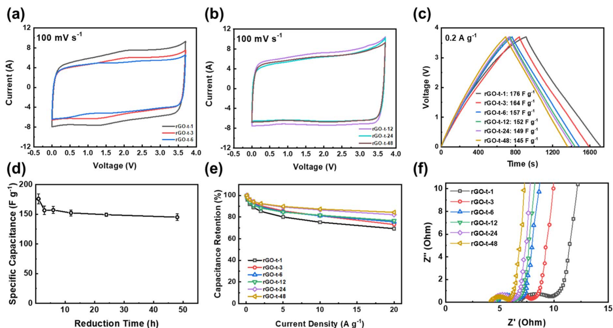
Fig. 8 CV curves at voltage sweep rate of 100 mV s -1 of graphene synthesized with reduction time of (a) 1 h, 3 h, and 6 h; (b) 12 h, 24 h, and 48 h; (c) charge–discharge curves, (d) specific capacitance, (e) rate performance, and (f) Nyquist plots of supercapacitors with rGOs synthesized with different reduction times.
