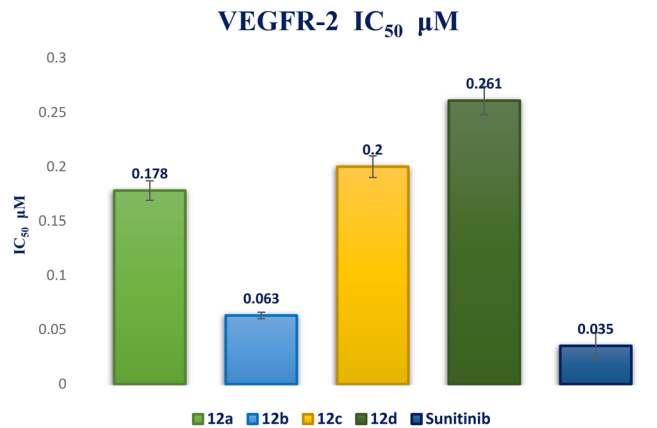
Fig. 6 IC 50 bar graph for compounds 12a–d against VEGFR-2 in comparison to sunitinib.
