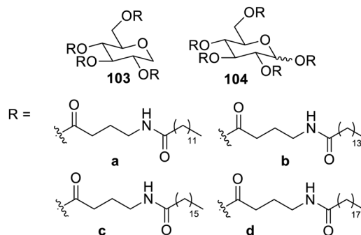
Fig. 64 Ester derivatives of GABA and (1,5-AG) and (Glc).
