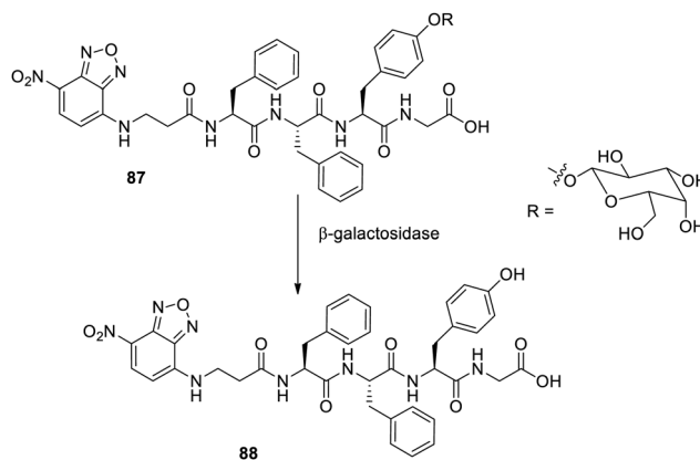
Fig. 56 Gelator precursor for \beta -galactosidase.
