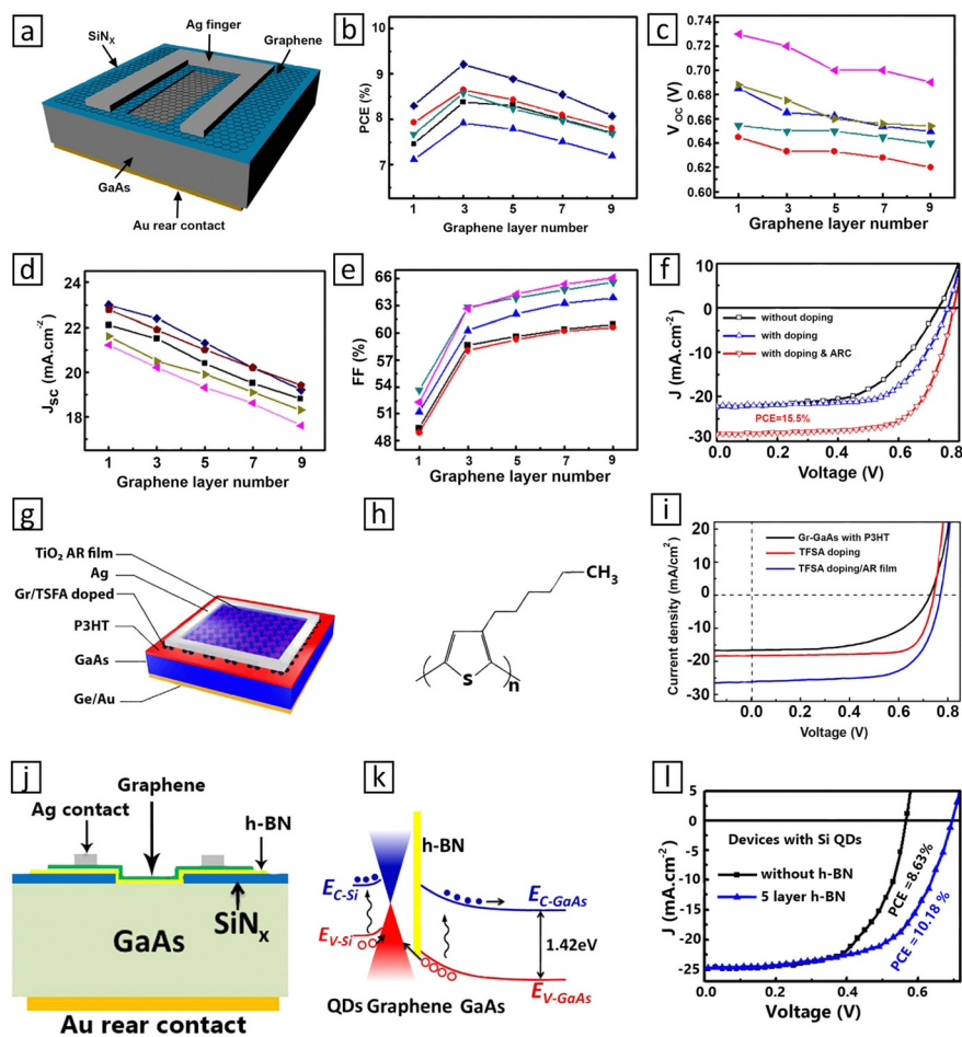
Fig. 15 (a) Schematic configuration of the graphene/GaAs solar cell. Five groups of characteristic (b) PCE, (c) V_{oc} , (d) J_{sc} , and (e) FF of the devices with various numbers of graphene layers. (f) J - V characteristics of the devices. Reproduced from ref. 171, with permission from Elsevier. (g) Schematic diagram of the TiO_2 -coated Gr-P3HT-GaAs solar cell after TFSA doping. (h) The structure of P3HT. (i) J - V characteristics of the Gr-P3HT-GaAs solar cell recorded in the initial state with TFSA doping and with TFSA doping/AR film. Reproduced from ref. 173, with permission from Elsevier. (j) Energy band diagrams of the graphene/h-BN/GaAs solar cell with Si QDs. (l) Schematic illustration of the graphene/h-BN/GaAs solar cell. (k) J - V characteristics of devices with Si QDs presented photo-induced doping. Reproduced from ref. 174, with permission from ref. 174. ©The Optical Society.
