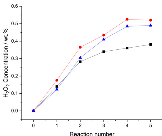
Fig. 3 Comparison of catalytic activity, over sequential H 2 O 2 synthesis reactions. Key: 0.5%Pd/TiO 2 (black squares), 0.25%Pd–0.25%Au/TiO 2 (red circles), 0.25%Pd–0.25%Sn/TiO 2 catalysts (blue triangles) H 2 O 2 direct synthesis reaction conditions: catalyst (0.01 g), H 2 O (2.9 g), MeOH (5.6 g), 5% H 2 /CO 2 (420 psi), 25% O 2 /CO 2 (160 psi), 0.5 h, 20 °C, 1200 rpm.
