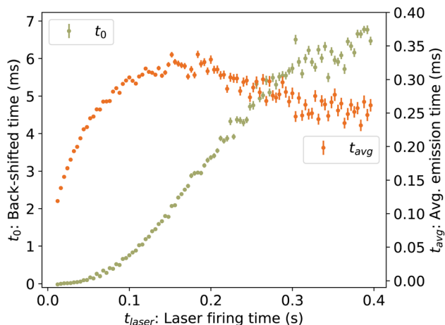
Fig. 6 (Left axis) Back-shifted times t_0 to which the vibrational energy distribution is re-heated following photon absorption at time t_{\text{laser}} , determined from laser-induced decay curves R_e(t_{\text{after}}) . (Right axis) Average emission times t_{\text{avg}} .
