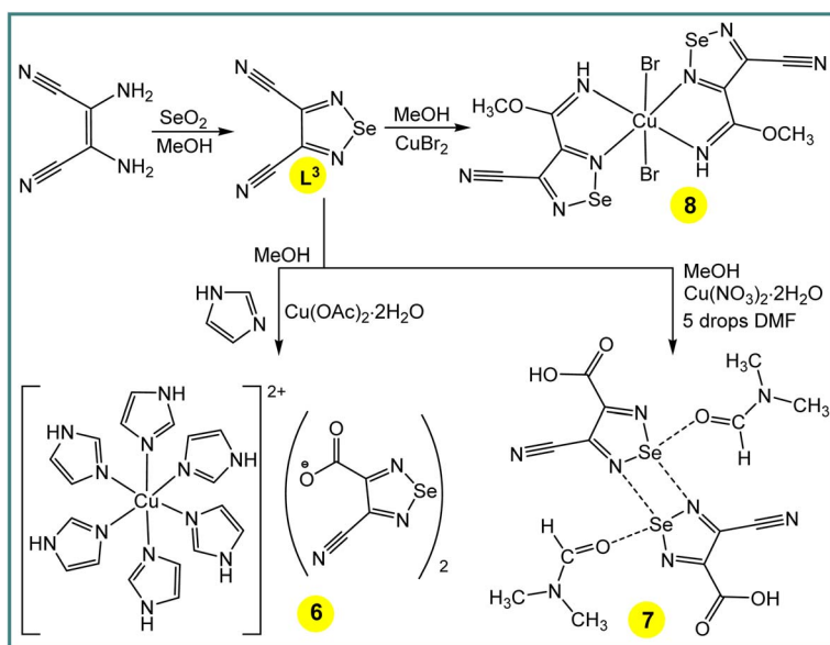
Scheme 4 Copper(II)-mediated transformation of one nitrile group of L 3 .
