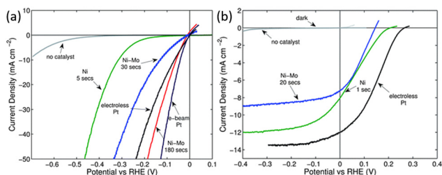
Fig. 12 (a) Polarization data of the HER activities of various catalysts on p + -Si microwire electrodes, (b) polarization data of the HER activities of various catalysts on illuminated p + -Si microwire array photoelectrodes. Reproduced with permission from ref. 69, Copyright © The Royal Society of Chemistry 2011.
