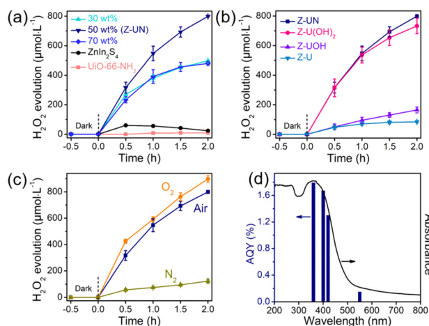
Fig. 1 Photocatalytic H 2 O 2 evolution over ZnIn 2 S 4 , UiO-66-NH 2 and ZnIn 2 S 4 /UiO-66-NH 2 hybrids with 30, 50, 70 wt% of UiO-66-NH 2 (a), Z-U, Z-UOH, Z-U(OH) 2 and Z-UN (b), photocatalytic H 2 O 2 evolution over Z-UN in O 2 , air and N 2 (c), AQYs of photocatalytic H 2 O 2 evolution using Z-UN at different wavelengths and UV-vis DRS of Z-UN (d). Reaction conditions: 20 mg photocatalysts, 40 mL deionized water, 400–780 nm illumination for (a)–(c), ambient air for (a), (b) and (d), ambient temperature.
