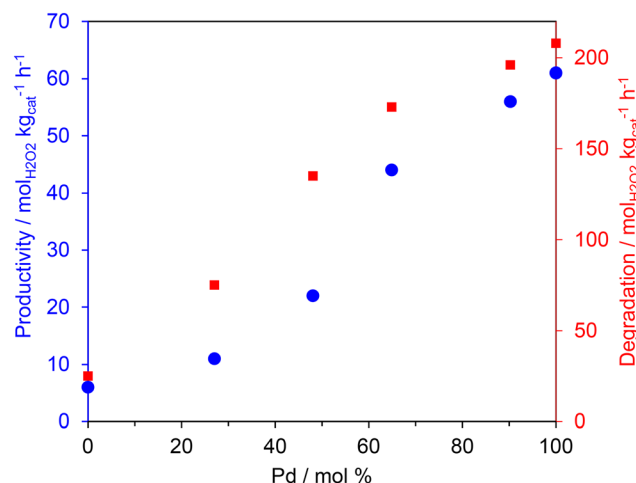
Fig. 1 The effect of Pd: Au ratio on the catalytic activity of 0.66% PdAu/TS-1 catalysts towards the direct synthesis (●) and subsequent degradation (■) of H 2 O 2 . H 2 O 2 direct synthesis reaction conditions: catalyst (0.01 g), H 2 O (2.9 g), MeOH (5.6 g), 5% H 2 /CO 2 (420 psi), 25% O 2 /CO 2 (160 psi), 0.5 h, 2 °C, 1200 rpm. H 2 O 2 degradation reaction conditions: catalyst (0.01 g), H 2 O 2 (50 wt% 0.68 g), H 2 O (2.22 g), MeOH (5.6 g), 5% H 2 /CO 2 (420 psi), 0.5 h, 2 °C, 1200 rpm.
