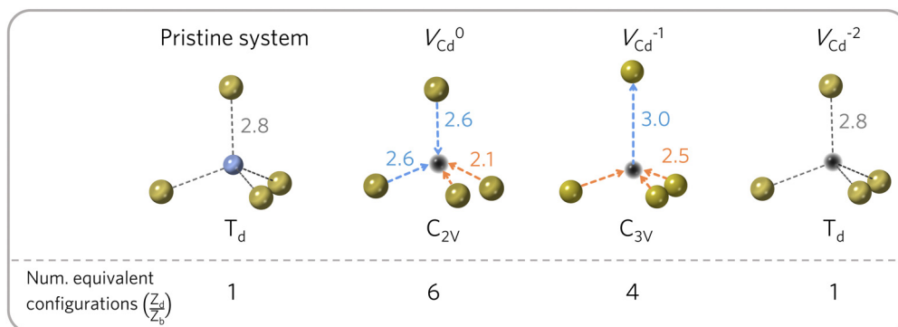
Fig. 3 Orientalional degrees of freedom for the cadmium vacancy in CdTe. The distortion undergone by the different charge states determines the number of symmetry-equivalent configurations ( Z_d^{\text{orient}}/Z_b^{\text{orient}} ). Cd in blue, Te in gold and vacancy in black. For each configuration, different colours are used to group bonds with equal distances (in Å), illustrating the defect site symmetry. Adapted from ref. 50.
