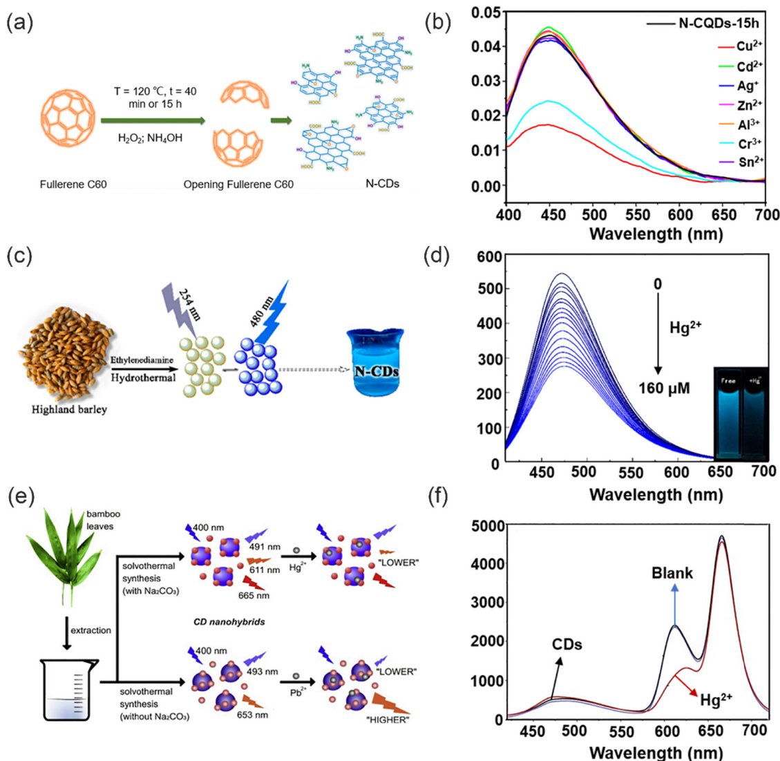
Fig. 8 The synthesis of CDs via top-down (or bottom-up) and their fluorescence response to heavy metal ions. (a) Preparation of fluorescent N-CDs. (b) The fluorescence spectra of N-CDs-15 h in the presence of different metal ions. Reproduced from ref. 81 with permission from Multidisciplinary Digital Publishing Institute Copyright 2021. (c) The preparation of the N-CDs. (d) The fluorescence response of the N-CDs under different concentrations of \text{Hg}^{2+} . Reproduced from ref. 88 with permission from Multidisciplinary Digital Publishing Institute. Copyright 2019. (e) Synthesis of dual- and three-emission CD nanohybrids for ratiometric fluorescent sensing of \text{Pb}^{2+} and \text{Hg}^{2+} , respectively. (f) Fluorescence spectra of the three-emission CD nanohybrids before and after its application for the analysis of a blank sample. Reproduced from ref. 89 with permission from Elsevier B.V. Copyright 2019.
