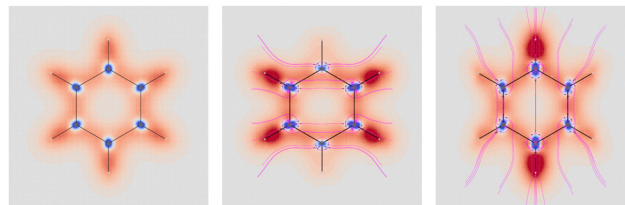
Fig. 2 EDPD of benzene over the molecular plane. Left \aleph_{av} ; center and right in-plane components. Trajectories (in magenta) of the current density (13) induced by the time derivative of the electric field are superimposed to the in-plane components. See caption to Fig. 1 for other details.
