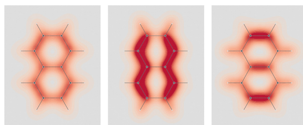
Fig. 3 EDPD of naphthalene over a plane located at 1 a.u. below the molecular plane. Left \aleph_{av} ; center and right in-plane components. See caption to Fig. 1 for other details.
