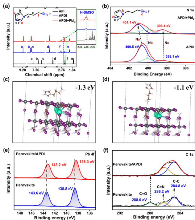
Fig. 1 (a) ^1\text{H} -NMR spectra of API, APDI and APDI + \text{PbI}_2 . (b) XPS spectra of N 1s for APDI and APDI + \text{PbI}_2 . (c) and (d) Theoretical models of Cs/FA-based perovskite with molecular surface interaction of \text{Pb}^{2+} with APDI. XPS spectra of (e) Pb 4f and (f) C 1s for perovskites with and without APDI.
