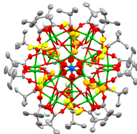
Fig. 2 Solid-state structure of \text{Cu}_{31} -oxo cluster 4 . Cu = green, O = red, C = grey, N = blue, H = very pale blue (non-coordinated/H-bonded \text{p}^{\text{r}}\text{OH} Cs = yellow, coordinated \text{p}^{\text{r}}\text{OH} Cs = orange). Ellipsoids displayed at 50% and hydrogen atoms (except OH) omitted.
