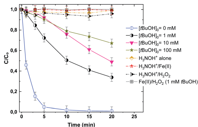
Fig. 4 Effect of tert -butanol ( t -BuOH) on the degradation kinetics of BF by the Fenton- \text{H}_3\text{NOH}^+ system (vol. = 200 mL, pH 3, temp. \sim 25^\circ\text{C} , C_0 = 20 \text{ }\mu\text{M} , [\text{Fe(II)}]_0 = 0.05 \text{ mM} , [\text{H}_2\text{O}_2]_0 = 0.5 \text{ mM} , [\text{H}_3\text{NOH}^+]_0 = 0.5 \text{ mM} , [\text{t-BuOH}]_0 = 1\text{--}100 \text{ mM} ).
