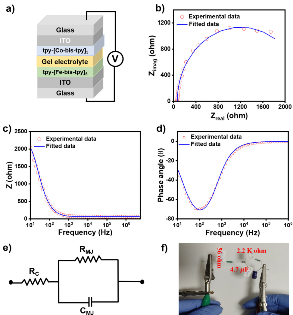
Fig. 7 (a) A schematic description of a molecular junction composed of ITO/tpy-[Fe(bis(tpy)) 5 ]/gel electrolyte/[Co(bis(tpy)) 5 ]-tpy/ITO. (b) The Nyquist plot of the junction. (c and d) Bodes plot at varying frequencies. (e) The Randles equivalent circuit and (f) a real circuit for the experimental validation of the fitted model.
