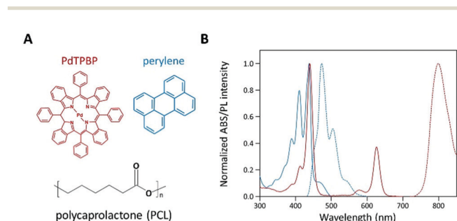
Fig. 1 (A) Molecular structures of PdTPBP (sensitizer), perylene (acceptor), and PCL (UC host material). (B) Normalized absorption (solid) and emission (dashed) spectra: sensitizer (PdTPBP, red) and acceptor (perylene, blue) in a PCL film.
