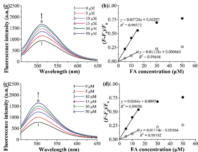
Fig. 8 (a and c) Fluorescence spectra of poly(m@NBD-MIP (a) and poly(m@NBD-MIP@lCPGMA@AuNPs (c) ( 0.25 \text{ mg mL}^{-1} ) upon their exposure to different concentrations of FA in ACN/DMF (4 : 1 v/v) at 25^\circ\text{C} for 2 h. (b and d) Dependence of the fluorescence enhancement of poly(m@NBD-MIP/CP (b) and poly(m@NBD-MIP/CP@lCPGMA@AuNPs (d) [MIP (filled symbols)/CP (open symbols)] on FA concentrations in ACN/DMF (4 : 1 v/v) at 25^\circ\text{C} (derived from (a), (c) and Fig. S8a, b, ESI†).
