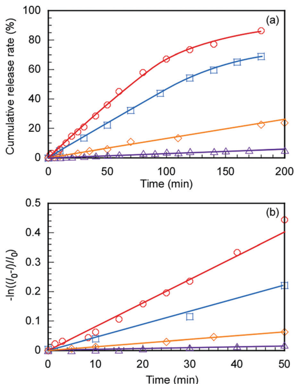
Fig. 8 (a) DOX release from DOX@C 70 /EUM at 25 °C ( \Delta ) and 50 °C ( \diamond ) and a blank solution without C 70 /EUM at 25 °C ( \square ) and 50 °C ( \circ ) in PBS. (b) -\ln((I_0 - I)/I_0) was plotted against dialysis time; I is the fluorescence intensity and I_0 is the initial intensity.
