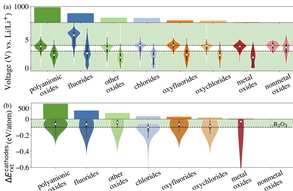
Fig. 2 (a) Distribution of the reduction and oxidation limits for each category that pass thermodynamic stability descriptor. (b) Distribution of the reaction energy \Delta E_{\text{rxt}} with \text{LiNiO}_2 , \text{LiCoO}_2 , \text{LiMn}_2\text{O}_4 and \text{LiFePO}_4 cathodes for each category that pass electrochemical stability descriptor. Both lithiated and half-lithiated cathodes are evaluated and the most negative \Delta E_{\text{rxt}} is selected as \Delta E_{\text{rxt}} with cathodes. The horizontal dash lines represent the limits of the descriptors. The histograms in (a) and (b) illustrate the numbers of compounds for each category that pass the descriptors.
