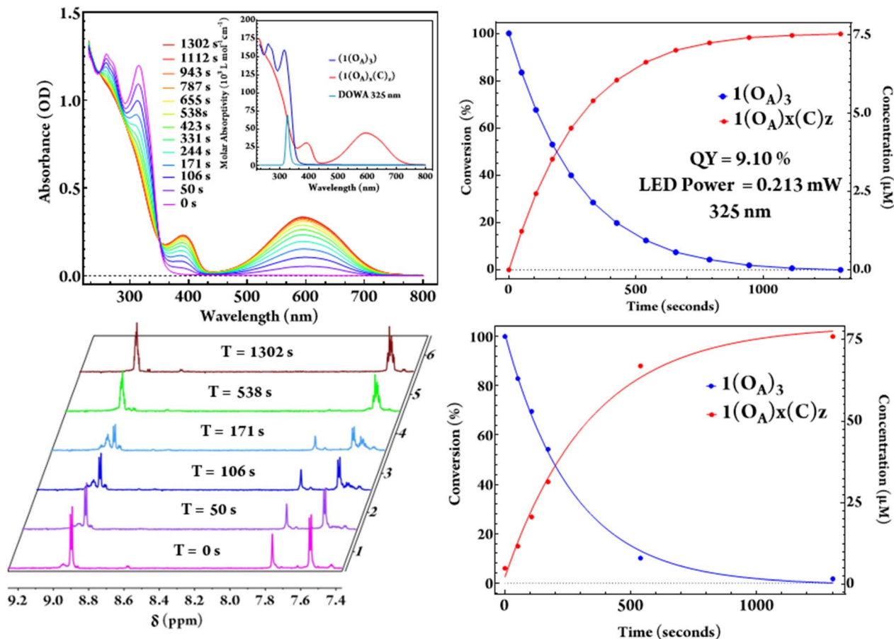
Fig. 4 Time-dependent UV-vis spectroscopy showing the photochemical conversion from (1(O A ) 3 ) to (1(C)) 3 in response to 0.21 mW of 325 nm light (upper panel) in dichloromethane with the corresponding 1 H NMR spectroscopy study (bottom), where x + z = 3.
