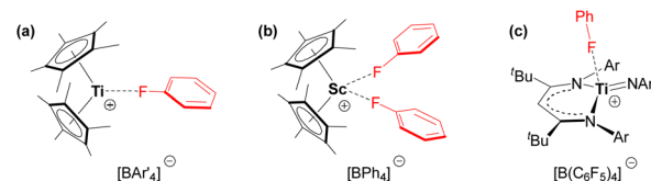
Fig. 7 Fluoroarene complexes of electrophilic transition metals. (a) [(Cp*) 2 Ti(κ 1 -FC 6 H 5 )]BAR' 4 ] (Ar' = Ph or C 6 F 5 ), (b) [(Cp*) 2 Sc(κ 1 -FC 6 H 5 ) 2 ][BPh 4 ], and (c) [(nacnac)Ti=NAr(κ 1 -FC 6 H 5 )]B(C 6 F 5 ) 4 ] (nacnac = {CH(C t Bu)NAr} 2 − ; Ar = 2,6-diisopropylphenyl). 56–58
