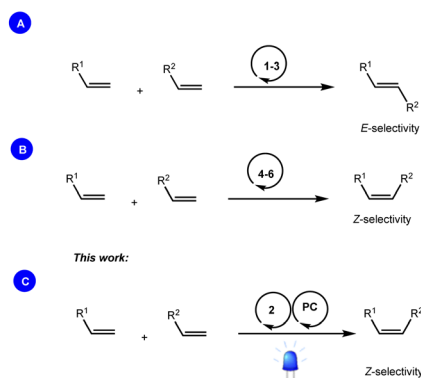
Scheme 1 Ru-based catalysts enabling stereoselective olefin cross-metathesis reactions.
