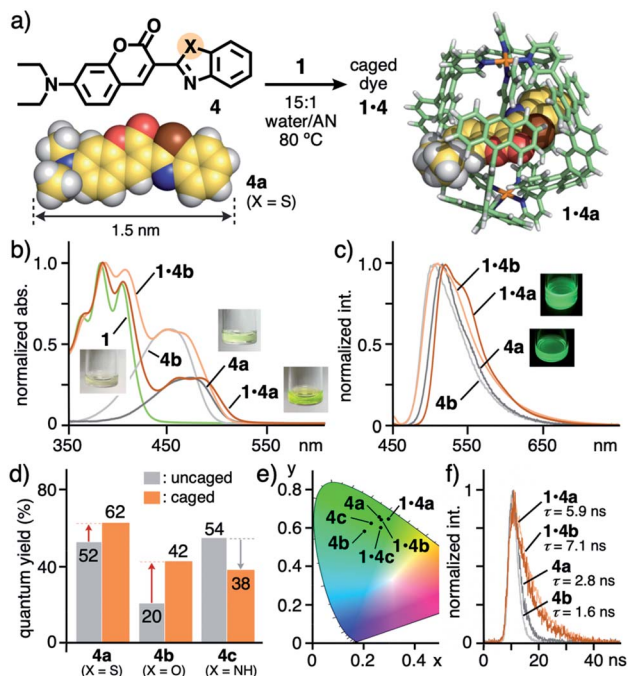
Fig. 3 (a) Formation of caged dyes 1·4 ( X = S, O , and NH ) and the optimized structures of 4a and 1·4a ( R^1 = H for clarity). (b) UV-visible spectra and photographs (r.t., 15 : 1 water/acetonitrile (AN)) of 1·4a , 1·4b , 1 , and 4a , 4b (in 2 : 1 water/AN), (c) their fluorescence spectra ( \lambda_{ex} = 450 nm) and (d) quantum yields, and (e) their CIE diagram (before and after binding by 1 ). (f) Fluorescence lifetimes (r.t., \lambda_{ex} = 355 nm, 15 : 1 or 2 : 1 water/AN) of 1·4a , 1·4b , and 4a , 4b .
