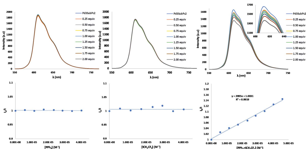
Fig. 4 Fluorescence quenching and plot of the quenching of 2 ( 2.14 \times 10^{-5} M in CH 2 Cl 2 ) versus: [PPh 3 ], left column; [CH 2 CF 3 ], middle column; and [PPh 3 + CH 2 CF 3 ], right column. Determination of the Stern–Volmer constant ( I/I_0 = 1 + K_{SV} \cdot x ).
