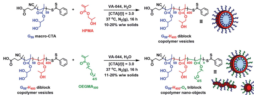
Scheme 1 Schematic illustration of the synthesis route employed for the preparation of poly(glycerol monomethacrylate) 59 -poly(2-hydroxypropyl methacrylate) 400 (G 59 -H 400 ) diblock copolymer vesicles at 10–20% w/w solids via RAFT aqueous dispersion polymerization of HPMA using a G 59 precursor, and their subsequent utilization as seed particles for the preparation of G 59 -H 400 -O x triblock copolymer nano-objects at 11–20% w/w solids via RAFT-mediated aqueous polymerization-induced disassembly (PIDA).
